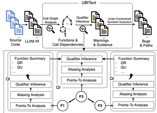
Figure 3: The workflow of UBITect, "QI":Qualifier Inference, "QR":qualifier requirements, "QU": qualifier updates
